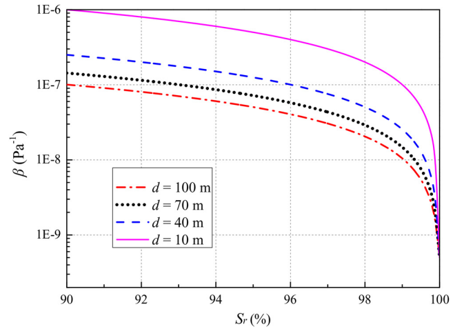
Fig. 5. Variation of the compressibility of pore fluid \beta with saturation degree S_r for different water depths.
