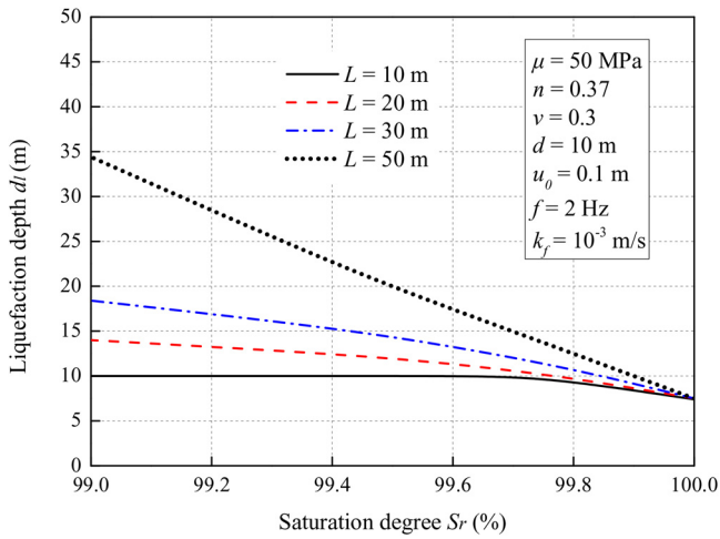
Fig. 8. Variation of liquefaction depth d_l with saturation degree S_r for different seabed thicknesses.
