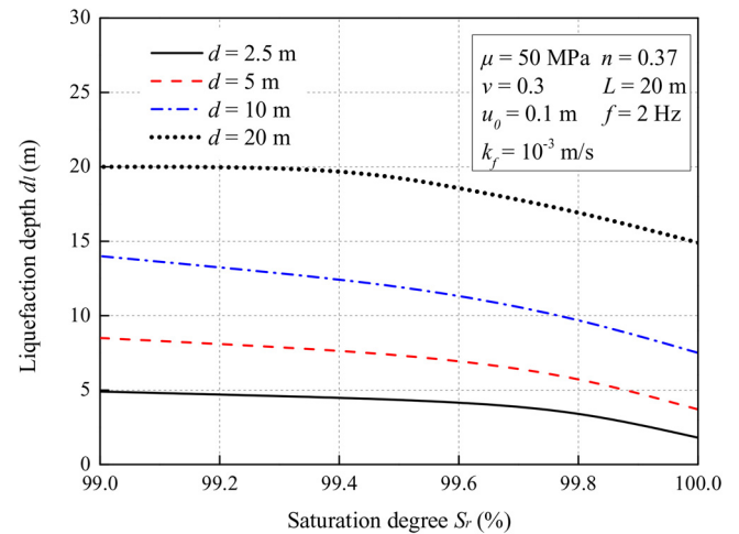
Fig. 7. Variation of liquefaction depth d_t with saturation degree S_r for different water depths.
