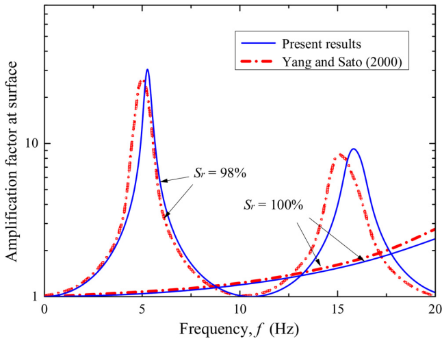
Fig. 2. Effects of frequency on the amplification factor of displacement at seabed surface when the seawater is removed (i.e., d=0 m).
