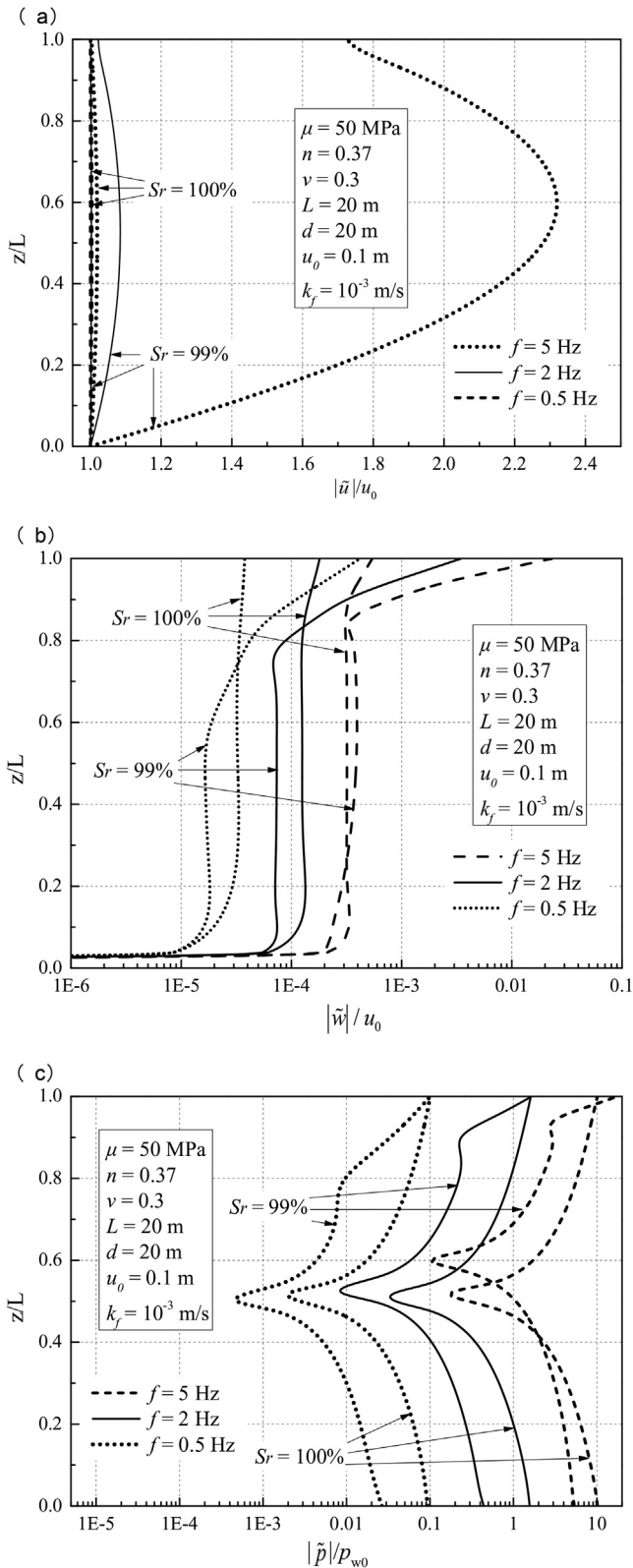
Fig. 4. Vertical distributions of (a) |\tilde{u}|/u_0 , (b) |\tilde{w}|/u_0 , and (c) |\tilde{p}|/p_{w0} versus the relative soil depth ( z/L ) for various excitation frequencies.
