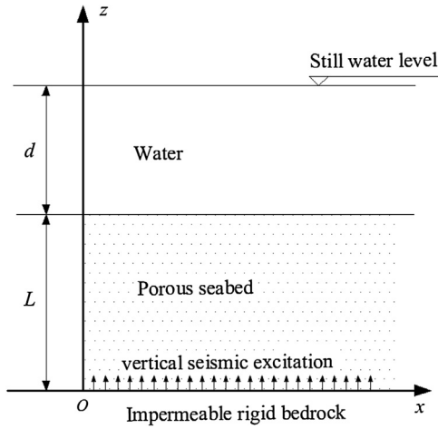
Fig. 1. Schematic diagram of the seismic problem.
