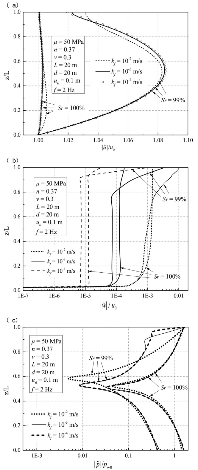
Fig. 3. Vertical distributions of (a) |\tilde{u}|/u_0 , (b) |\tilde{w}|/u_0 , and (c) |\tilde{p}|/p_{w0} versus the relative soil depth ( z/L ) for various soil permeabilities.
